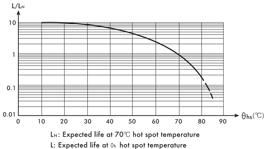
Expected life VS hot spot temperature at U_N
